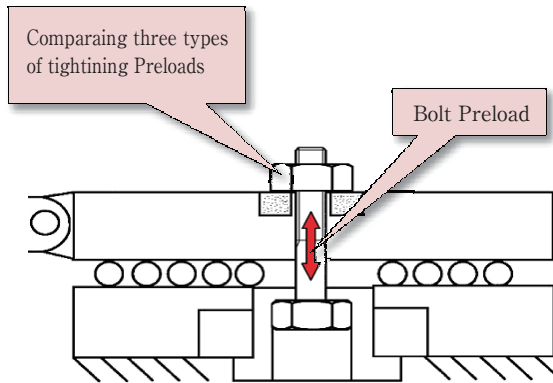
Comparison Loosening Test with set Amplitude Displacement at \pm 0.35\text{mm} and 3 different Preloads
