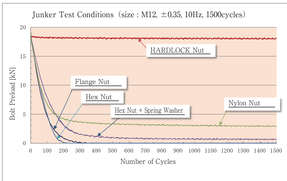
Various Nuts Comparison Test Results
