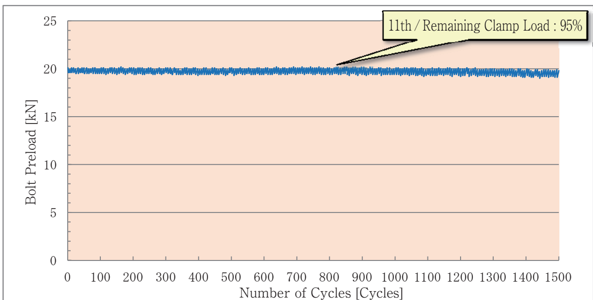
Junker Test Result after 11th Tightening
