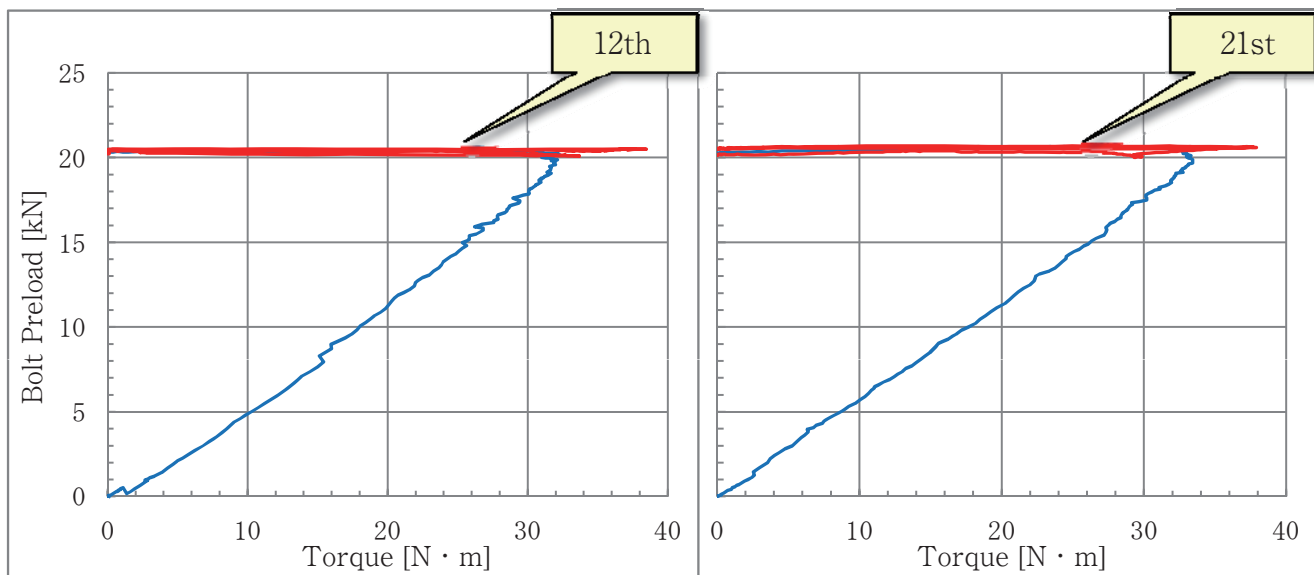
12th & 21st Tightening
