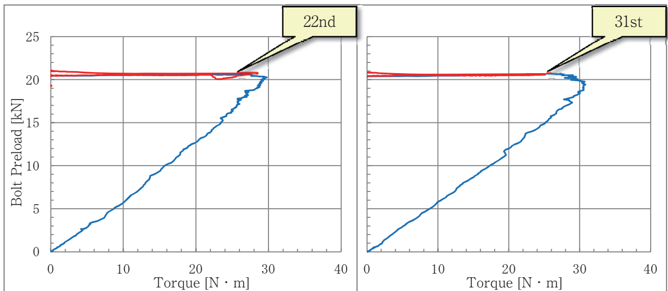
22nd & 31st Tightening
