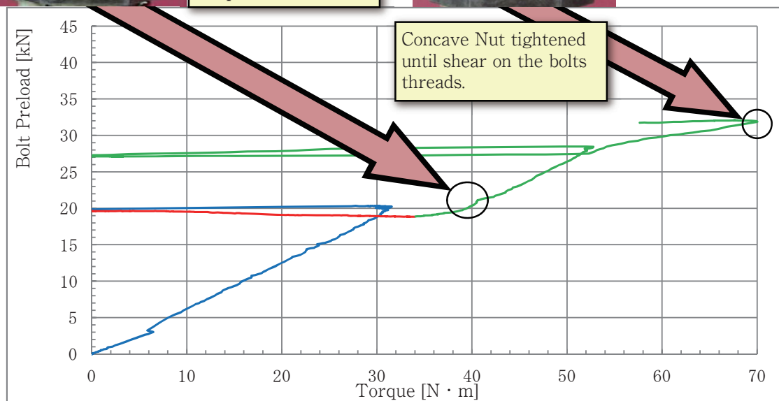
Graph (6) Double Nut (Upper) : Tightening until damage on the bolts threads
