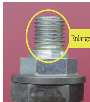
Graph (5) HARDLOCK Convex Nut : Tightening until damage on the bolts threads
