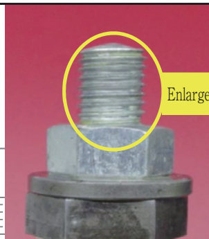
Graph (6) Double Nut (Upper) : Tightening until damage on the bolts threads
