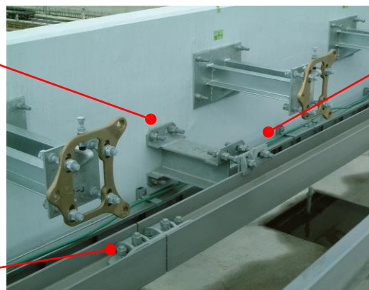
Guide Rail & H Beam M24 C4 HDZ35
