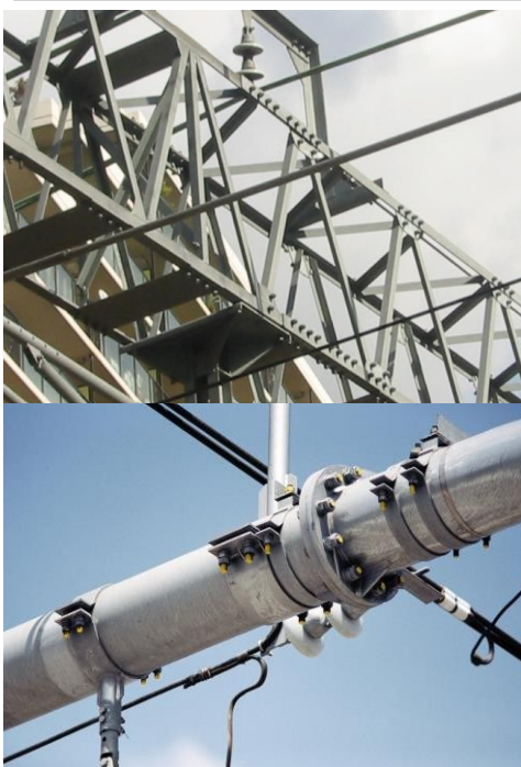
Truss & Beam flange M16, M20 C4 HDZ35
