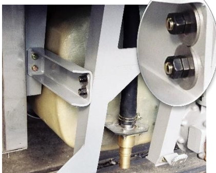
Fixing train car equipment M6, M8 C4
